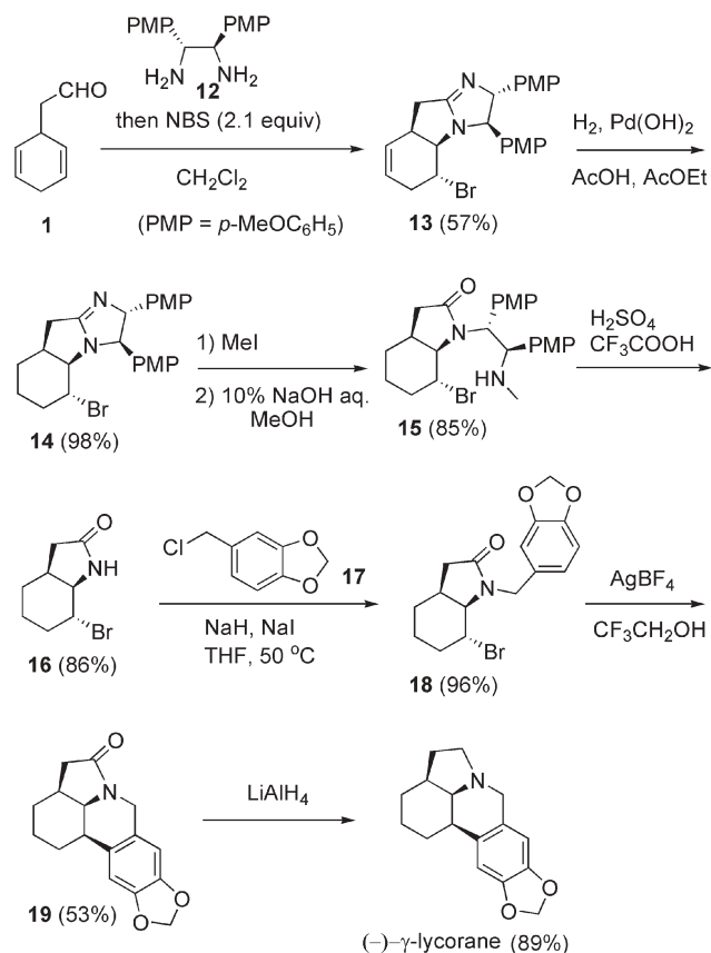
Scheme 6 Asymmetric synthesis of (–)- \gamma -lycorane.
