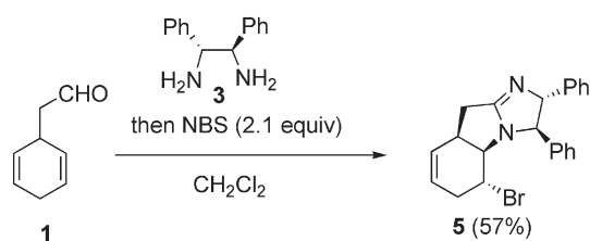
Scheme 5 One-pot operation.
